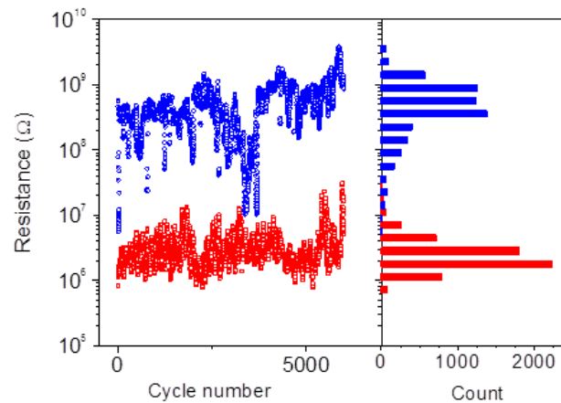
Fig. 3: R_{\text{High}} and R_{\text{Low}} states as a function of cycle number, recorded on a 10 \times 10 \mu\text{m}^2 device. The endurance reaches beyond 5000 cycles with a R_{\text{High}}/R_{\text{Low}} ratio \approx 1000 [3].
