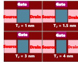
Fig. 3: Simulated SET Structures.
