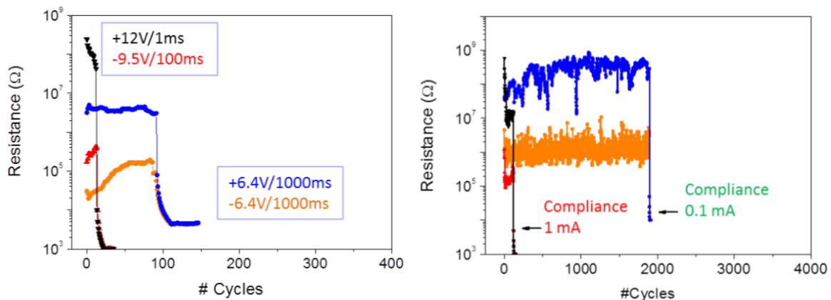
Fig. 2: Left : Endurance of 100 \times 100 \mu\text{m}^2 cells for different switching pulses: (-9.5\text{V}/100\text{ms} and +12\text{V}/1\text{ms}) pulses typically lead to an endurance < 50 cycles. Lower voltage but much longer duration (-6.4\text{V}/1000\text{ms} and +6.4\text{V}/1000\text{ms}) yields endurance < 150 cycles.
