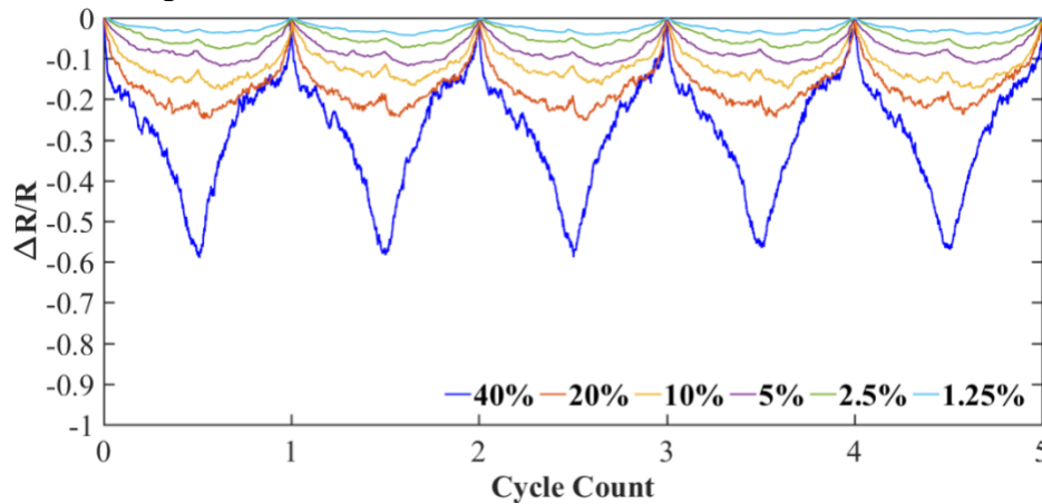
Fig1. 3 Sensing functions of porous CNF/PDMS (direct method) at 3% wt. CNF at different max compressive strains.
