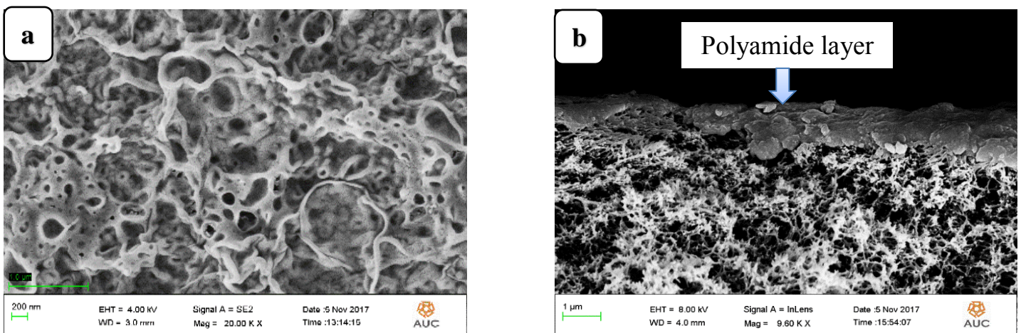
Fig. 1: SEM images of TFNC 0.01% including (a) Top surface, (b) Cross-section
