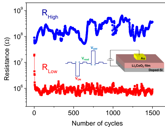
Fig. 1: Endurance measurement of a 100 \times 100 \mu\text{m}^2 {Au / \text{Li}_x\text{CoO}_2 / doped Si} device. The inset shows the shape of pulses used to switch the device and to measure R_{\text{Low}} and R_{\text{High}} (at a lower read voltage).
